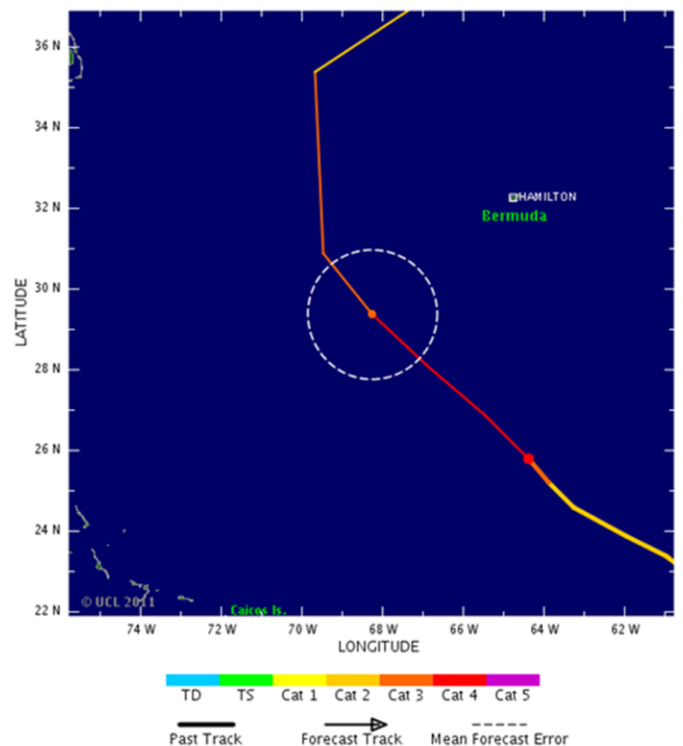
Hurricane Path uncertainty in 33 hours
